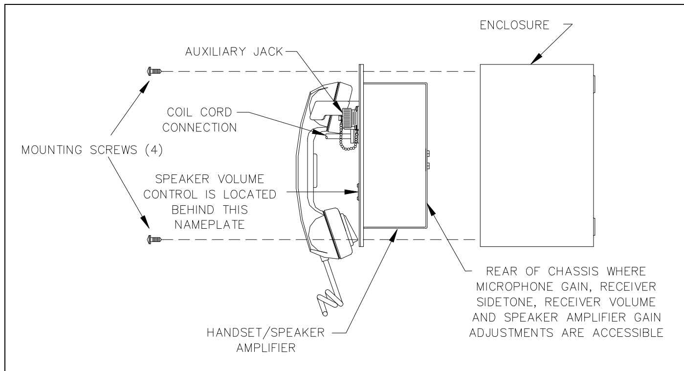
Figure 1. Installation and Adjustment Details
